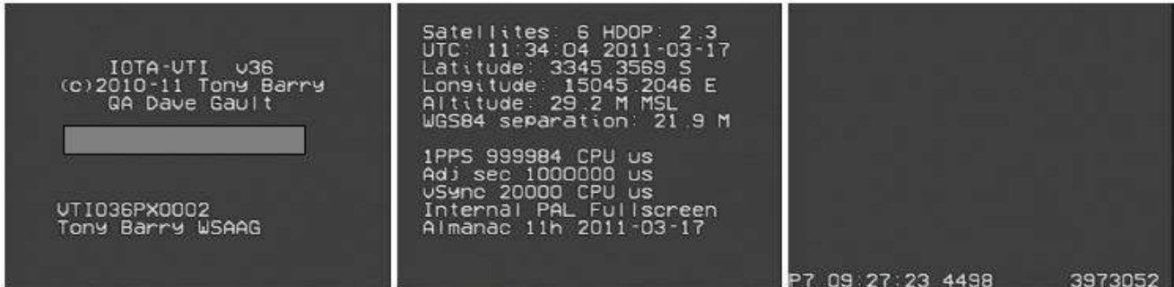
Splash screen
